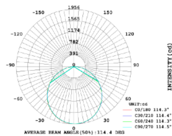
LUMINOUS INTENSITY DISTRIBUTION
